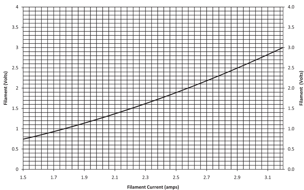
HPC-225-FB V-A Curve
